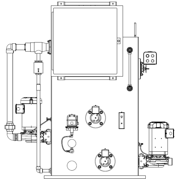
TYPICAL C-5 UNIT
